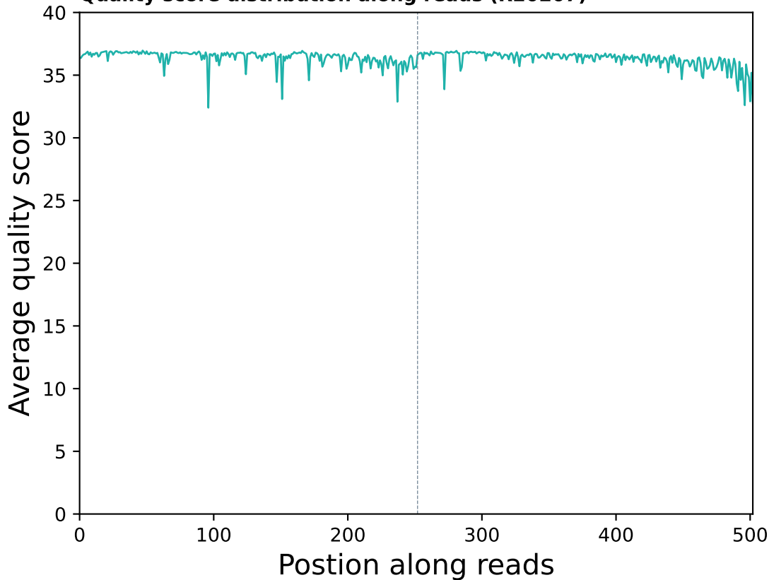
Quality score distribution along reads (R20207)
